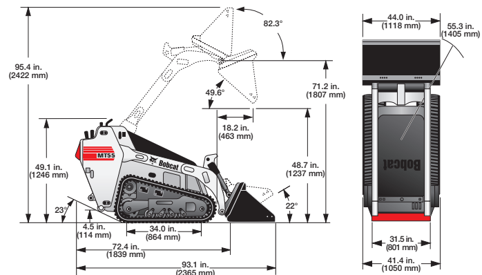
MT55 with optional 10" Track:
