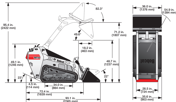
Standard MT52 and MT55 Dimensions:
